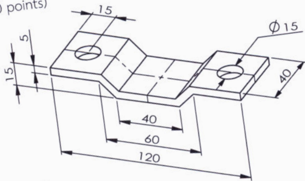
Figure 4: Trimetric projection view. (Scale 1:2)
