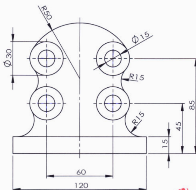
Figure 1: Front view (Scale 1:2)
